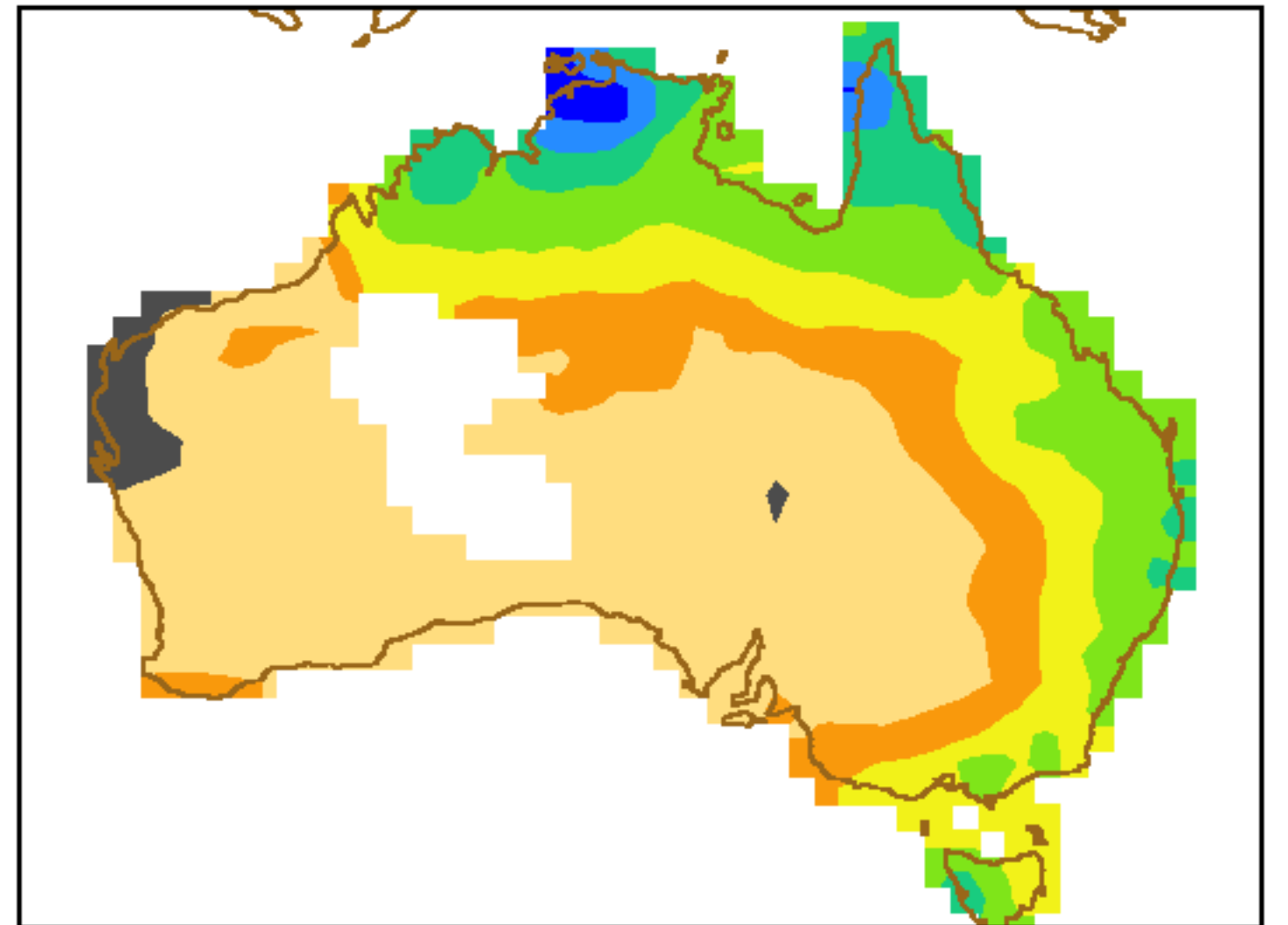
Normal weekly rainfall in NDJ (mm)
