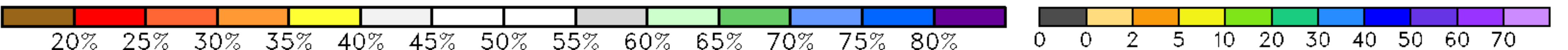
Chance of exceeding normal weekly rainfall
