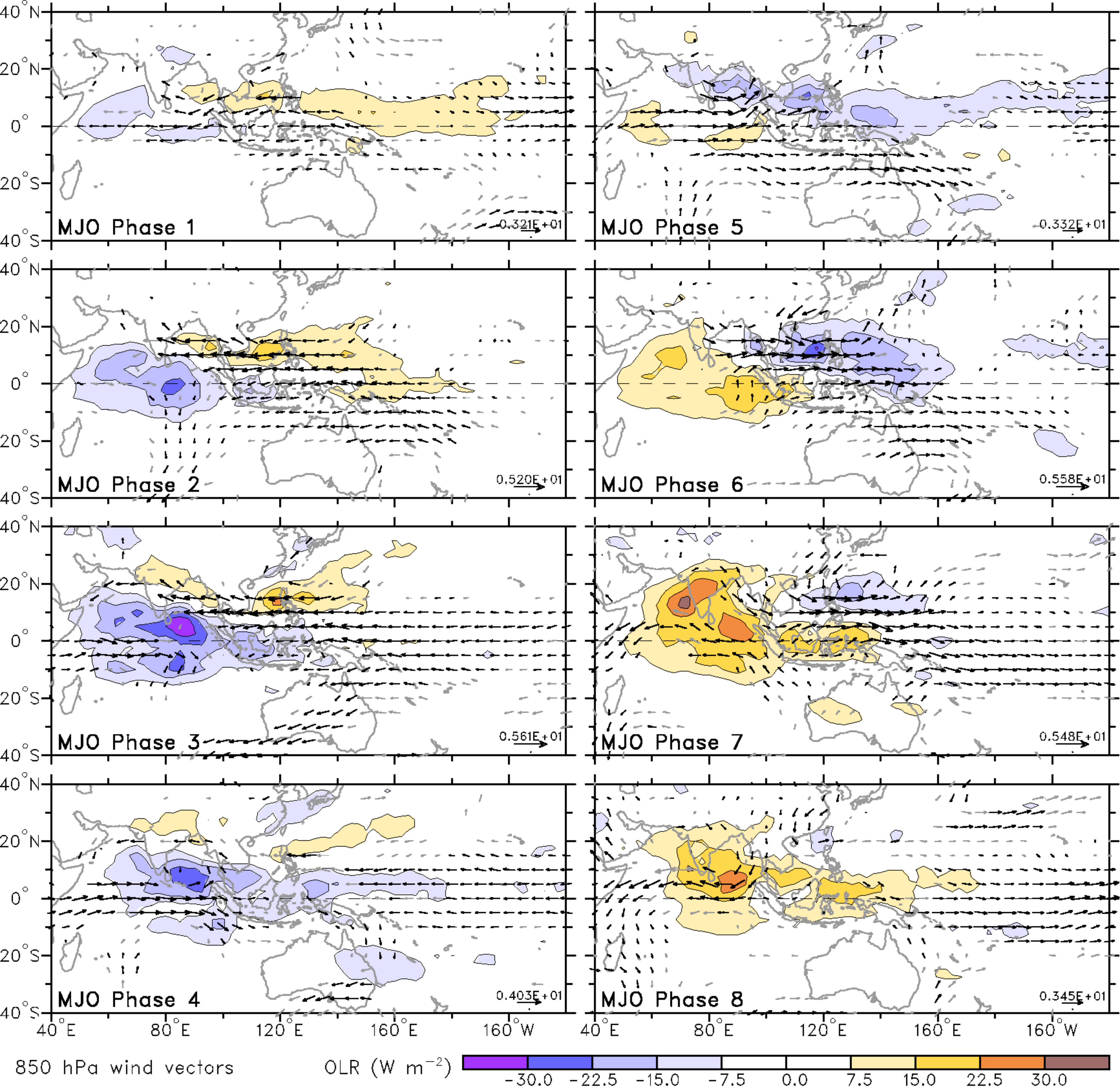
MJO average conditions in May-Jun-Jul, 1974-2009
