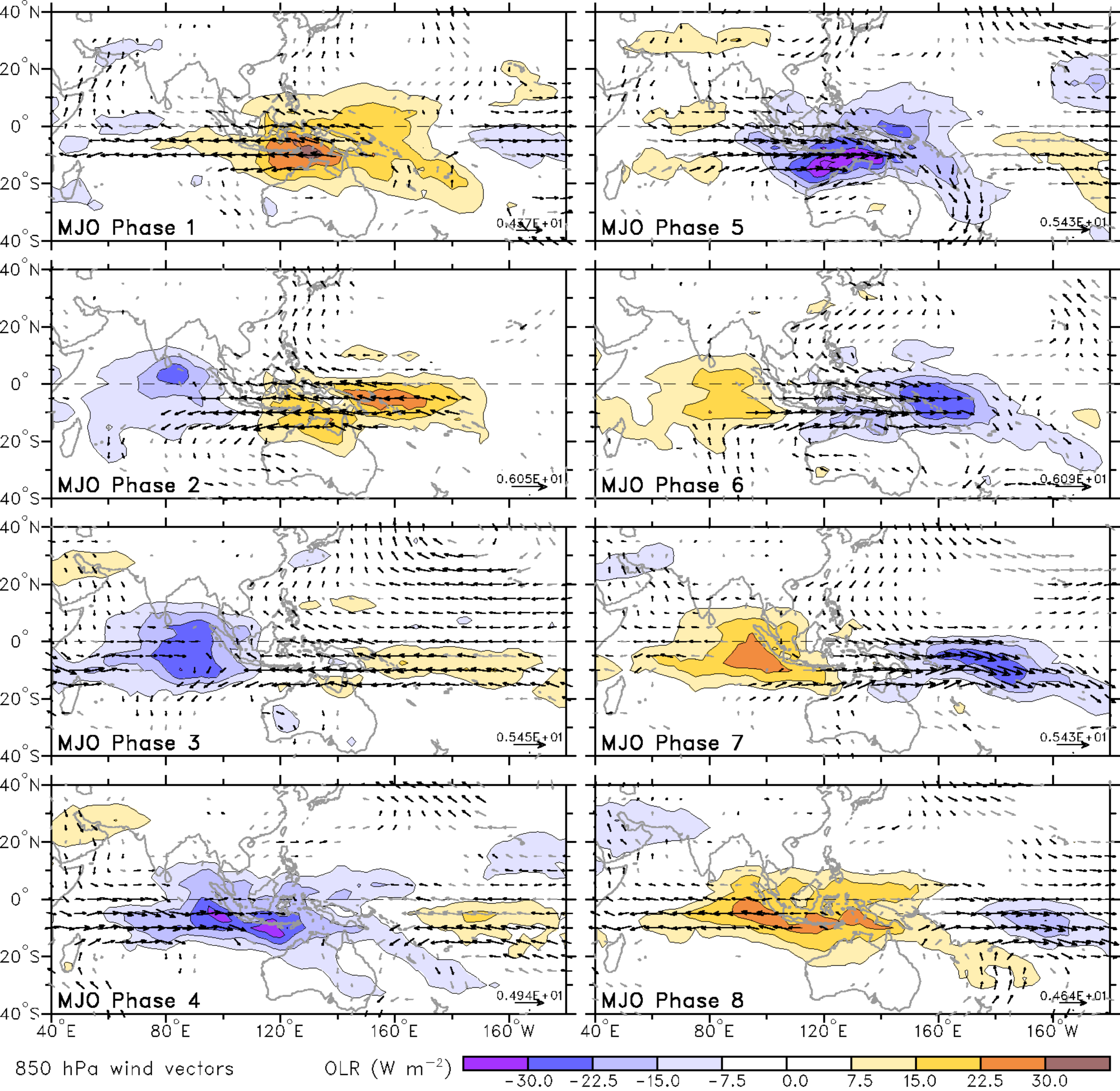
MJO average conditions in Jan-Feb-Mar, 1974-2009
