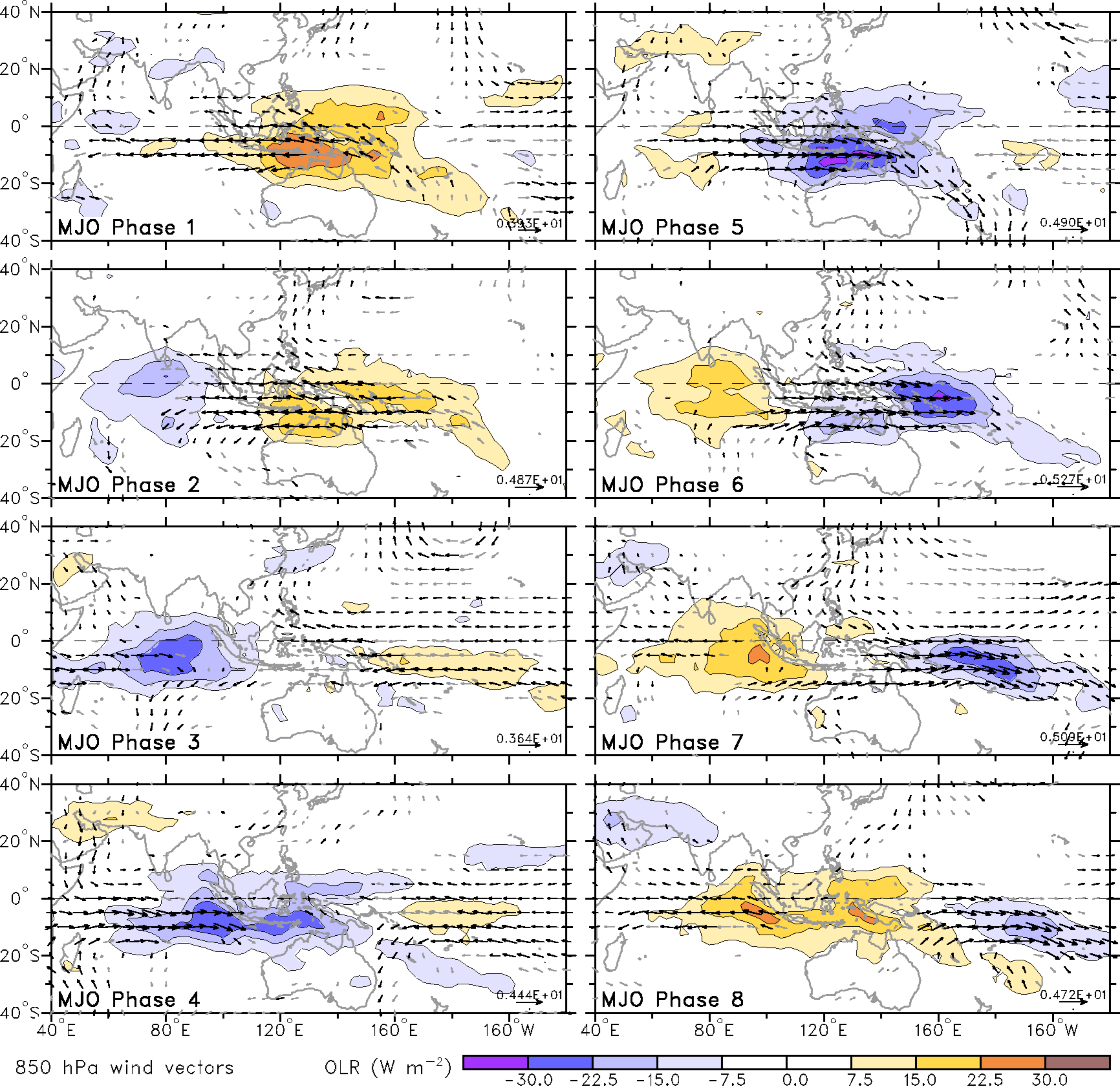
MJO average conditions in Feb-Mar-Apr, 1974-2009
