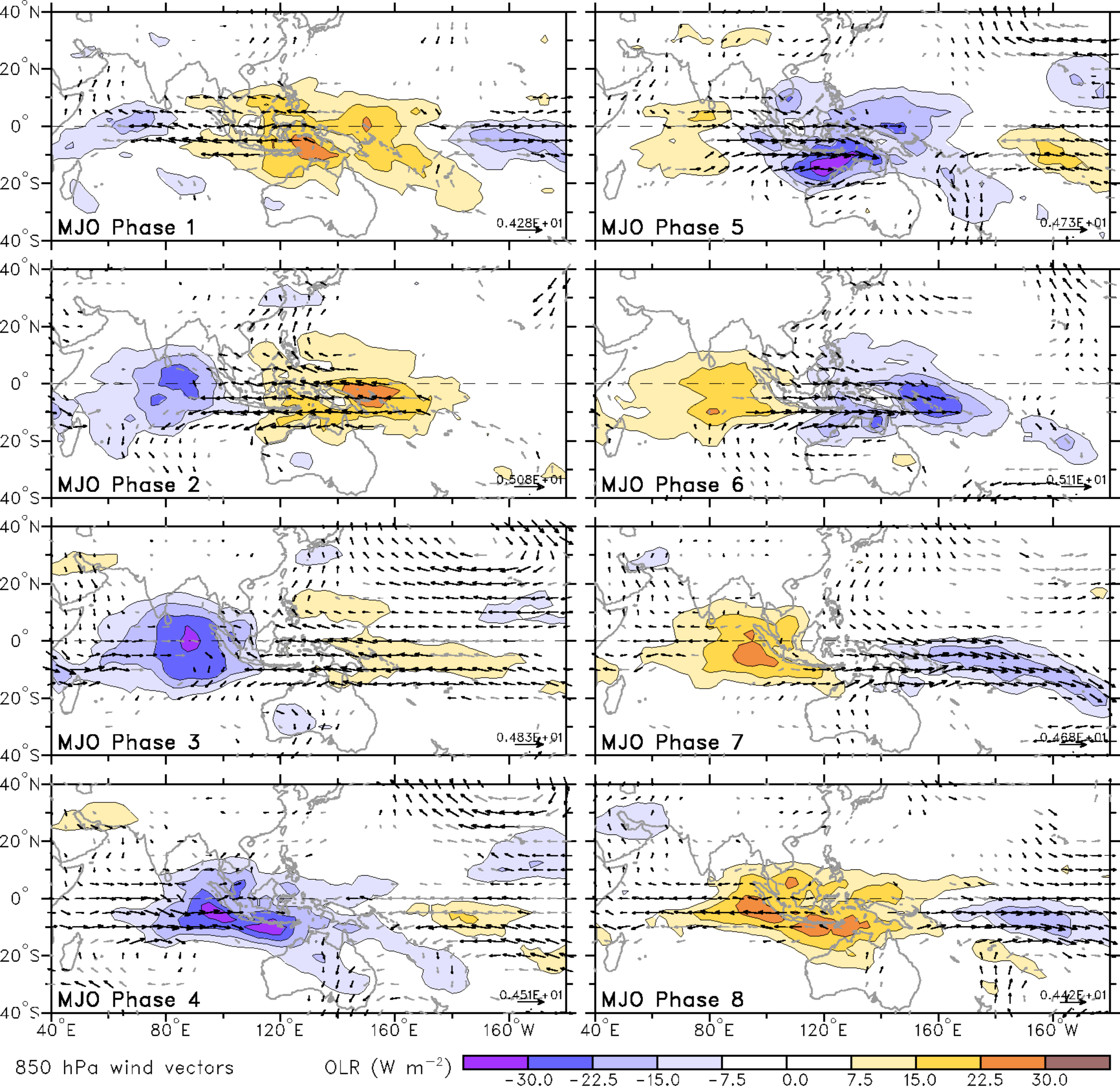
MJO average conditions in Dec-Jan-Feb, 1974-2009
